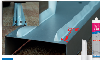
4 Applying adhesive
